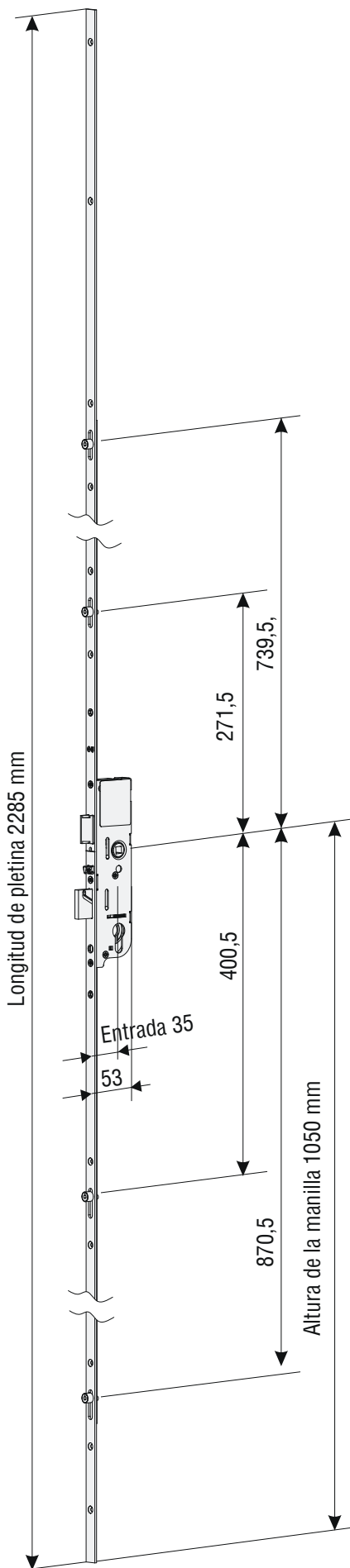
Cerradero Central FERCOMATIC
